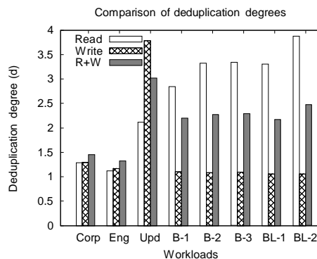
Fig. 1. Comparison of deduplication degree for different workloads. Note the different profiles for read-heavy and write-heavy workloads.
