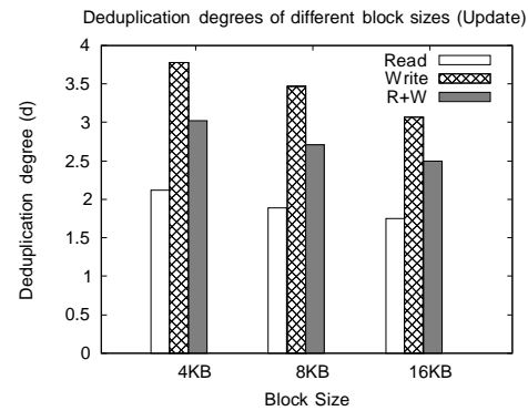
Fig. 4. Deduplication degree as a function of block size for the Upd trace. Other traces show similar trends.
