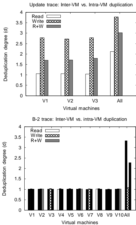
Fig. 2. Intra-VM vs. inter-VM deduplication for the Update and B-2 traces. Other boot traces show similar profile. The Vx bars shows the intra-VM deduplication for each VM, while the All bar shows the inter-VM deduplication when all VMs share the same cache.
