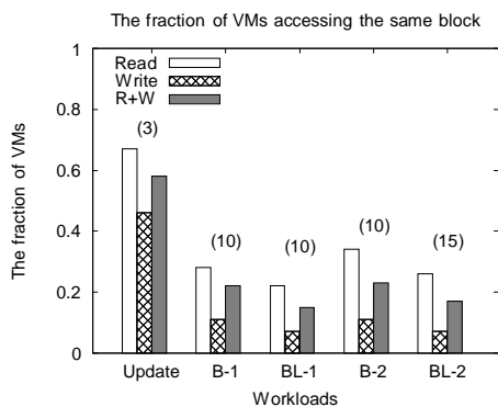
Fig. 3. The (number) shows the total number of VMs. A small fraction of VMs access the same block because of VM-unique content.
