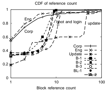
Fig. 5. CDF of block reference counts for all studied traces.
